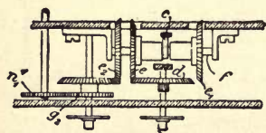
Fig. 348.—Aron Meter—Plan of Reversing Mechanism
